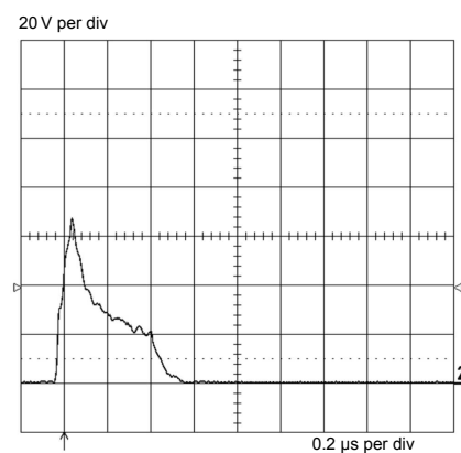
Figure 10. ESD response at V_{PP} = 15 kV air discharge (ESDA25-4BP6)
