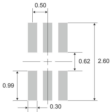
Figure 12. Footprint recommendations, dimensions in mm
